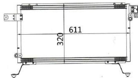
CAR MODEL: MITSUBISHI PAJERO YEAR: 00-05 SIZE: 611x320x16
