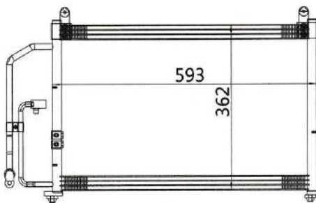
CAR MODEL: DAEWOO LANOS I & II YEAR: 97~02 SIZE: 593x362x16
