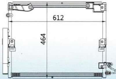
CAR MODEL: TOYOTA Land Cruiser /Lexus LX470 YEAR: 98-08 SIZE: 612×464×16
