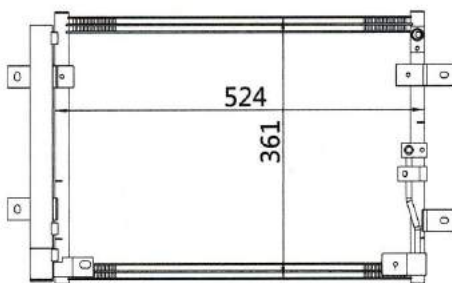
CAR MODEL: KIA BONGO YEAR: 2000 SIZE: 524x361x16
