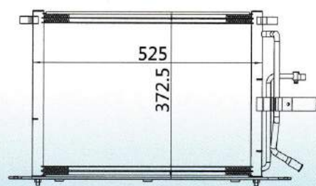
CAR MODEL: FORD FIESTA YEAR: 94-97 SIZE: 525x372.5x20
