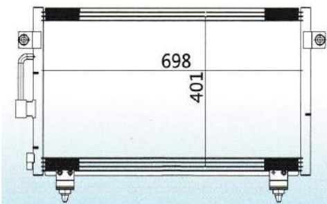
CAR MODEL: CHERY TIGGO YEAR: 2009 SIZE: 698x401x20
