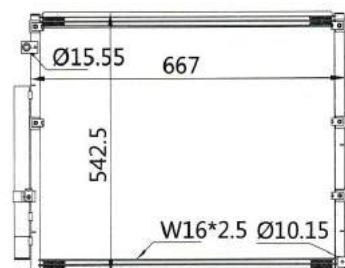
CAR MODEL: TOYOTA LANDCRUISER UZJ100 4700 YEAR: 99-07 SIZE: 667x542x16
