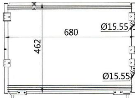
CAR MODEL: Town Ace / Noah CR4 YEAR: 96-01 SIZE: 680×462×16
