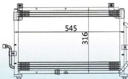
CAR MODEL: MATIZ I YEAR: 94-97 SIZE: 545x316x16
