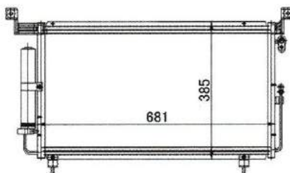
MODEL: 哈飞赛马 YEAR: SIZE: 681x385x16
