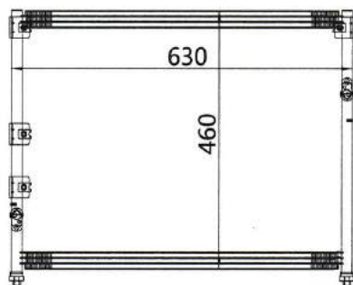
CAR MODEL: MAZDA MPV HMC6472 YEAR: SIZE: 630x460x16
