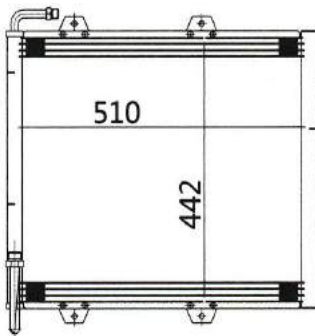
MODEL: 江铃双排座 YEAR: SIZE: 510x442x20
