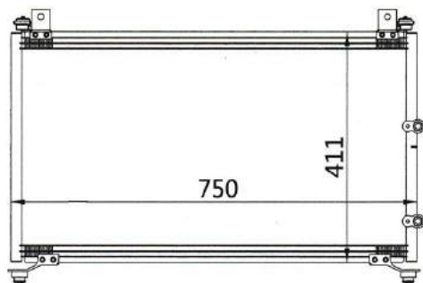
CAR MODEL: HONDA STEPWAGON YEAR: 1996 SIZE: 750×411×16
