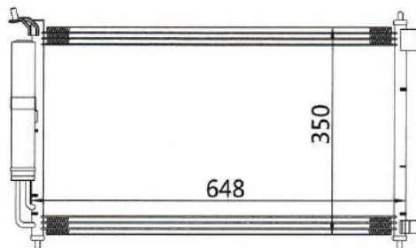
CAR MODEL: NISSAN Tiida C11 YEAR: 04-07 SIZE: 648×350×16
