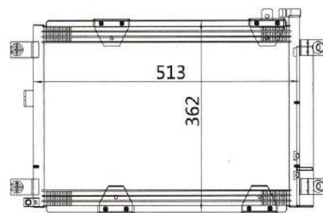
CAR MODEL: SUZUKI VITARA YEAR: 97-04 SIZE: 513x362x16
