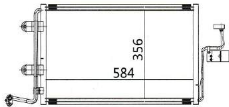
CAR MODEL: BORA(16) YEAR: 98 SIZE: 584x356x16
