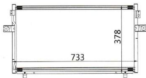
CAR MODEL: NISSAN CEFIRO-A32 R12 YEAR: SIZE: 733×378×16
