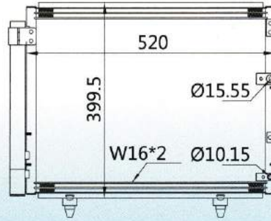
CAR MODEL: TOYOTA YEAR: SIZE: 520×399.5×16
