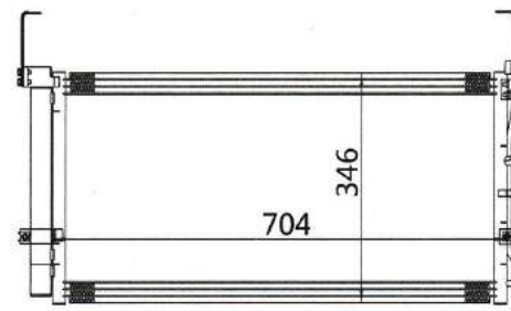
CAR MODEL: HYUNDAI SANTA FE YEAR: 01-06 SIZE: 704x346x16
