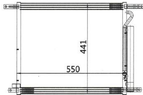
CAR MODEL: Hyundai Kalos YEAR: 2009 SIZE: 550x441x16
