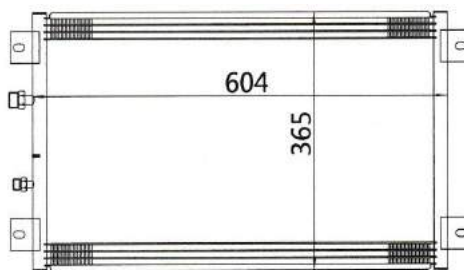
CAR MODEL: CATER PILLAR 320D YEAR: SIZE: 604x365x16
