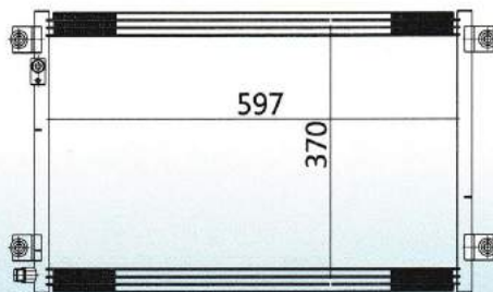
MODEL: 欧曼 ETX6 YEAR: SIZE: 597x370x16
