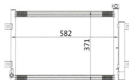
MODEL: 悍威 J5 重卡 (带瓶) YEAR: SIZE: 582x371x20
