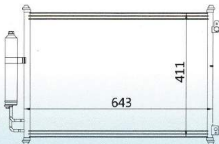
CAR MODEL : NISSAN X-Trail T30 YEAR: 08-11 SIZE: 643×411×16
