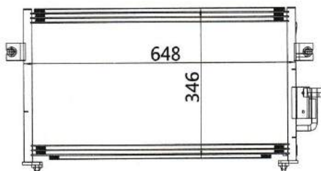
CAR MODEL: HYUNDAI ELANTRA I YEAR: SIZE: 648x348x16
