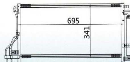
CAR MODEL: HYUNDAI SONATA YEAR: 06- SIZE: 695x341x16
