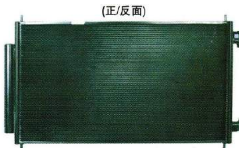
适用车型:CRV 年份:07款- 规格:709X383X16(波5mm) OEM:80110-SWA-A01
