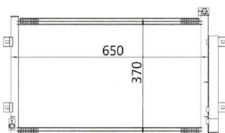
MODEL: 新大威淮柴重卡 YEAR: SIZE: 650x370x20
