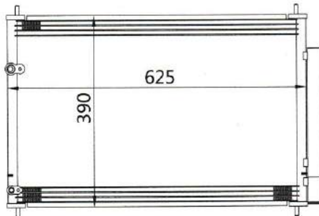
CAR MODEL: TOYOTA AXIO NEW ALTIS YEAR: SIZE: 625×390×16
