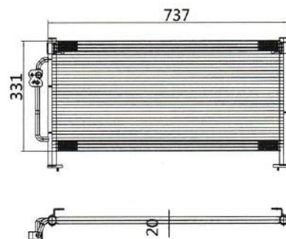
CAR MODEL: SUBARU FORESTER YEAR: 97 SIZE: 737×331×20
