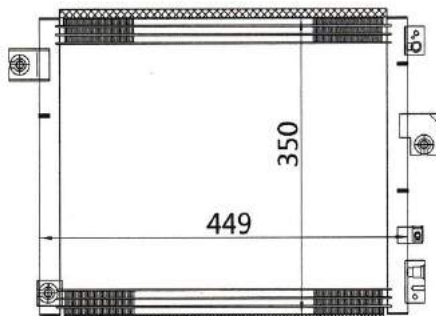
CAR MODEL: HYUNDAI ATOS N/M YEAR: SIZE: 449x350x20
