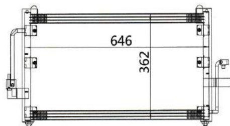
CAR MODEL: DAEWOO NUBIRA II YEAR: 99- SIZE: 646x362x16
