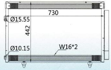
CAR MODEL: TOYOTA Highlander YEAR: 00-03 SIZE: 730×442×16
