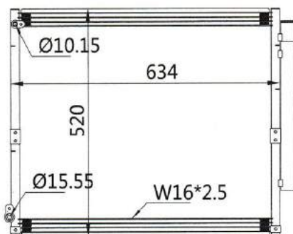
CAR MODEL: Toyota 4Runner YEAR: 03-09 SIZE: 634x520x16
