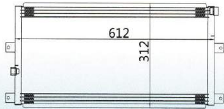
CAR MODEL: TOYOTA Kijang Diesel r134a YEAR: 97-99 SIZE: 612x312x16
