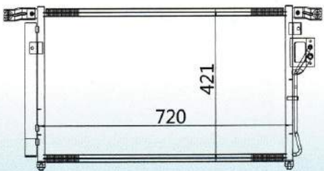
CAR MODEL: HYUNDAI SANTA FE YEAR: 07-09 SIZE: 720x421x16
