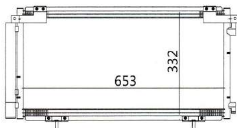
CAR MODEL: SUBARU LAGECY BD YEAR: 95-98 SIZE: 653×332×16
