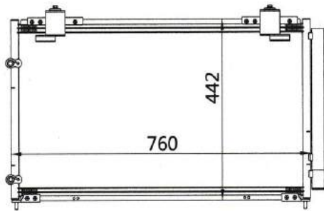
CAR MODEL: HONDA ODYSSEY YEAR: 99-/02/04 SIZE: 760×442×16
