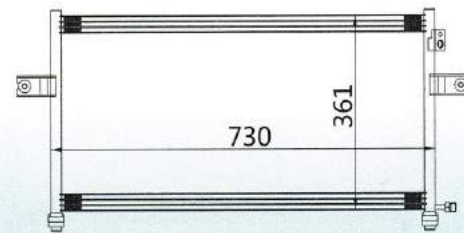
CAR MODEL: NISSAN PRIMERA-P12 YEAR: 02-08 SIZE: 730×361×16
