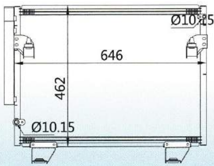
CAR MODEL: HILUX/VEGA YEAR: 05- SIZE: 646×462×16
