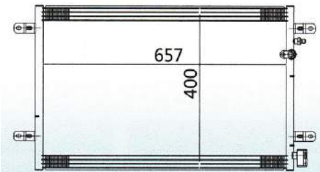
CAR MODEL: AUDI A6 YEAR: SIZE: 657x400x16
