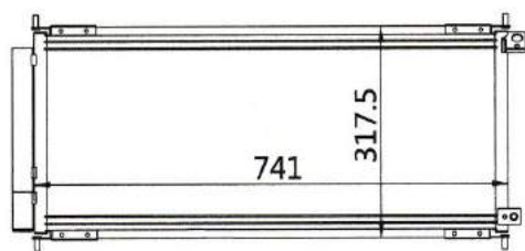
CAR MODEL: HONDA FIT YEAR: 07-08 SIZE: 741×317×16
