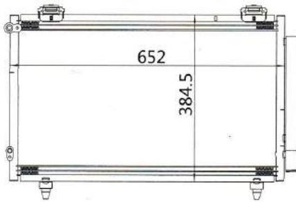
CAR MODEL: TOYOTA COROLLA/MATRIX /ALTIS YEAR: 03-04 SIZE: 652x384.5x16
