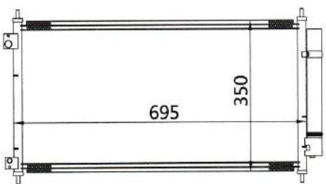
CAR MODEL: HONDA ACCORD YEAR: 08 SIZE: 695×350×16
