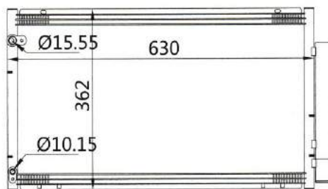
CAR MODEL: TOYOTA COROLLA/MATRIX YEAR: 07-08 SIZE: 630×362×16
