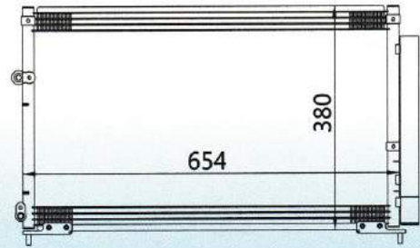
CAR MODEL: HONDA CIVIC FA1 YEAR: 94-97 SIZE: 654×380×16
