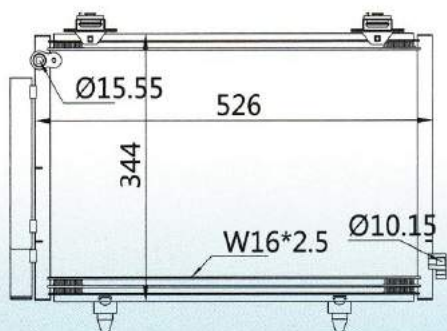
CAR MODEL: TOYOTA COROLLA YEAR: 02- SIZE: 526×344×16
