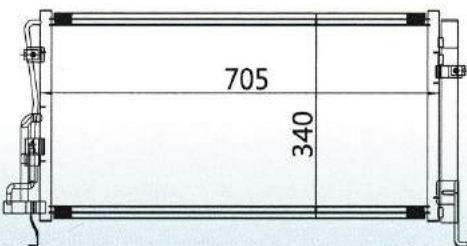
CAR MODEL: HYUNDAI SONATA YEAR: 03-04 SIZE: 705x340x16
