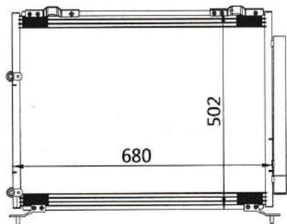
CAR MODEL: HONDA PILOT YEAR: 03-07 SIZE: 680×502×16
