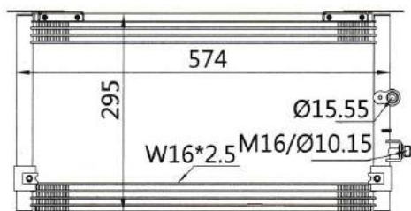
CAR MODEL: TOYOTA HILUX-2700 YEAR: 97-01 SIZE: 574×295×20
