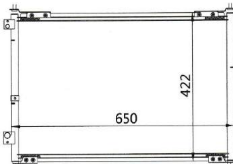
CAR MODEL: HONDA ODYSSEY RA6 YEAR: 94-03 SIZE: 650×422×16
