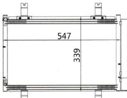
CAR MODEL: SUZUKI SWIFT YEAR: 06 SIZE: 547x339x16
