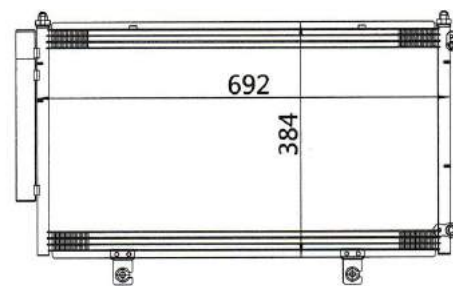
CAR MODEL: BYD F6 YEAR: SIZE: 692x384x16
