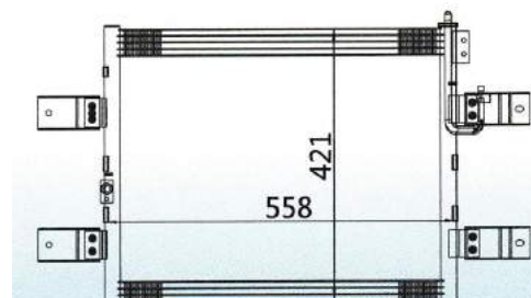
MODEL: 解放奥威 YEAR: SIZE: 558x421x20
