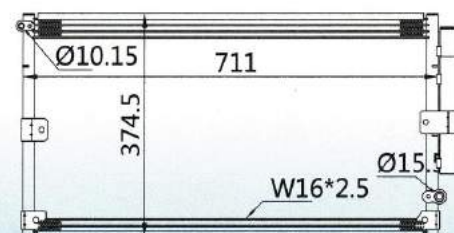
CAR MODEL: TOYOTA LANCRUISER YEAR: SIZE: 711×374×16
