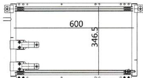
CAR MODEL: DADI YEAR: SIZE: 600x346.5x16
