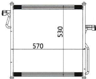
CAR MODEL: MAZDA B4000 PICKUP YEAR: SIZE: 570x530x16
