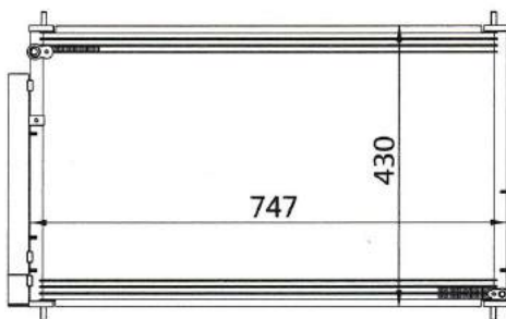
CAR MODEL: HONDA YEAR: 94-97 SIZE: 747×430×16
