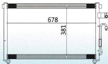
CAR MODEL: CHERY CROSS YEAR: SIZE: 678x381x20
