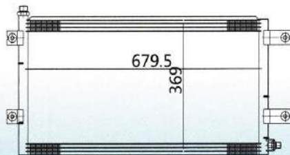
MODEL: 豪运 YEAR: SIZE: 679.5x369x20
