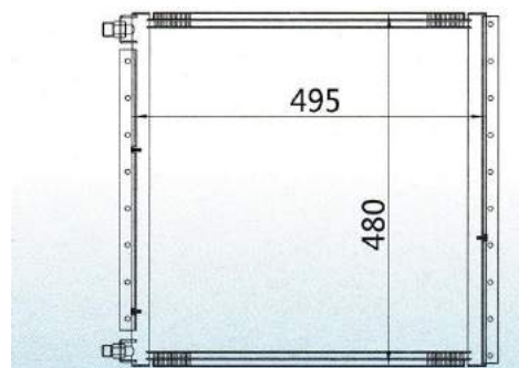
CAR MODEL: 19x21x20 R12 (2 厘 ) YEAR: SIZE: 495x480x20
