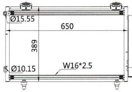
CAR MODEL: TOYOTA COROLLA ZZE YEAR: 00-01 SIZE: 650×389×16
