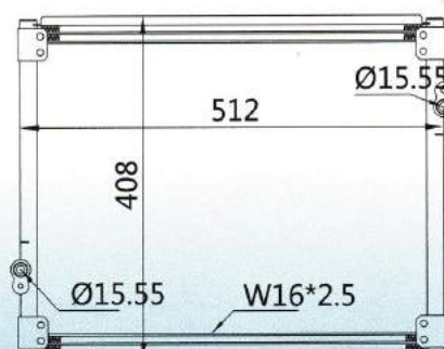
CAR MODEL: TOYOTA HIACE YEAR: SIZE: 512x408x16
