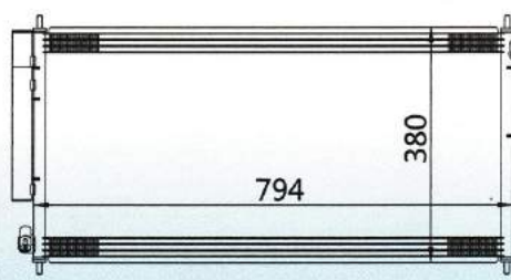
CAR MODEL: HONDA YEAR: 94-97 SIZE: 794×380×16
