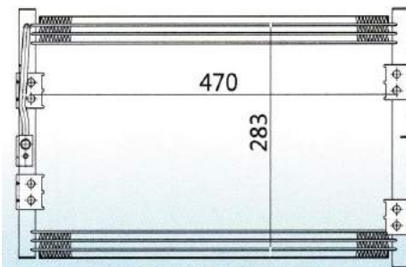
MODEL: 夏利三缸电喷 YEAR: SIZE: 470x283x16
