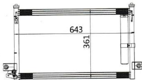
CAR MODEL: MITSUBISHI JEEP YEAR: SIZE: 643x361x20
