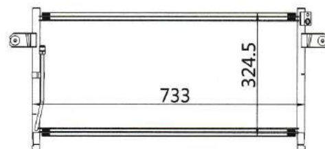
CAR MODEL: NISSAN PATROL/ Y61 YEAR: 92 SIZE: 733×324.5×16
