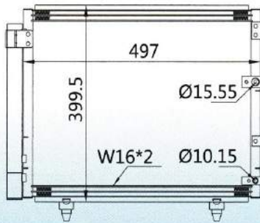
CAR MODEL: TOYOTA AVANZA(AT) YEAR: SIZE: 497×399×16
