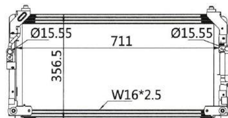
CAR MODEL: TOYOTA 4500/LANDCRUISER YEAR: 93-98 SIZE: 711×356×20
