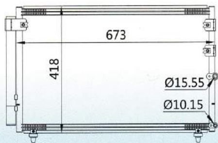
CAR MODEL: TOYOTA MARK II YEAR: 00- SIZE: 673×418×16
