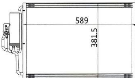
CAR MODEL: OPEL CORSA-C YEAR: 2000 SIZE: 589×381.5×16
