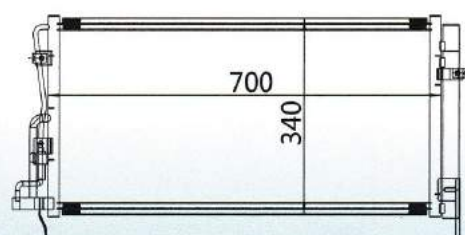
CAR MODEL: HYUNDAI YEAR: SIZE: 700x340x16
