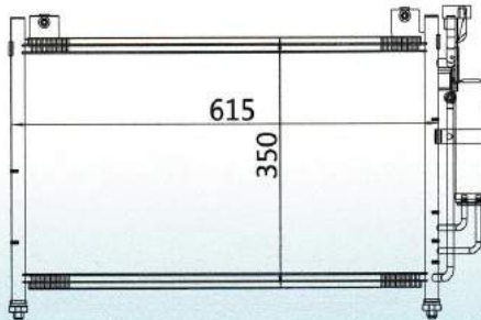
CAR MODEL: MAZDA 2 YEAR: SIZE: 615x350x16
