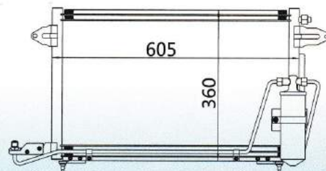
CAR MODEL: JATTA GT (WITH DIRER) YEAR: SIZE: 605x359.7x20
