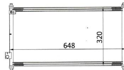
CAR MODEL: HONDA SM-X YEAR: 1996 SIZE: 648×320×16
