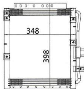
CAR MODEL: KIA PREGIO (SMALL) YEAR: SIZE: 348x398x20
