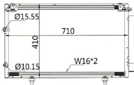
CAR MODEL: TOYOTA CAMRY 2.4/Camry ACV#01-06 YEAR: 01-06 SIZE: 710×410×16
