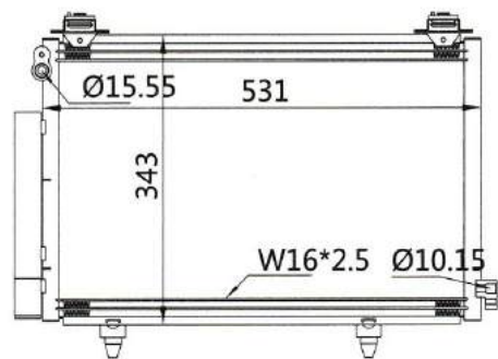
CAR MODEL: TOYOTA ECHO YEAR: 99-02 SIZE: 531×343×16
