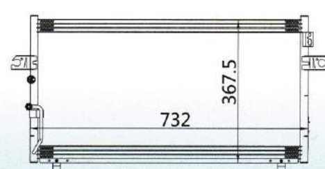
CAR MODEL: NISSAN MAXIMA/ INFINITI I35 YEAR: 02-04 SIZE: 732×367.5×16
