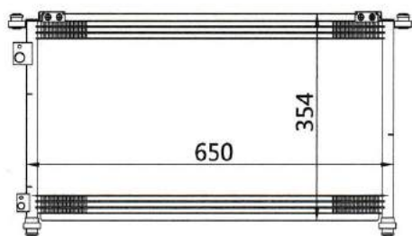
CAR MODEL: HONDA CIVIC 2.0 YEAR: SIZE: 650×354×16
