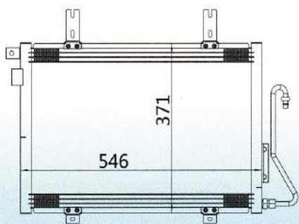
CAR MODEL: RENAULT KANGOO YEAR: 98-03 SIZE: 546x371x20
