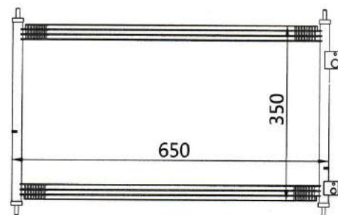
CAR MODEL: HONDA CIVIC (HYBRID) YEAR: 03-05 SIZE: 650×350×16
