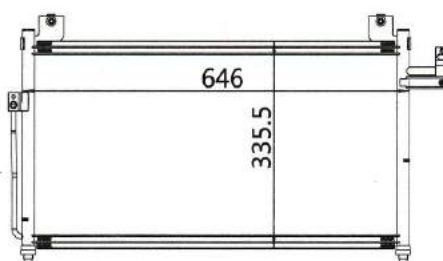
CAR MODEL: MAZDA PROTÉGÉ YEAR: 02-03/ 99-03 SIZE: 646x335.5x16
