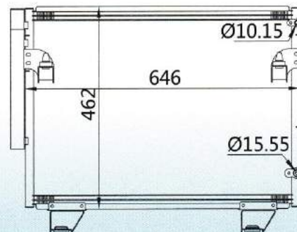
CAR MODEL: HILUX Diesel (05-) YEAR: 05-09 SIZE: 646×462×16
