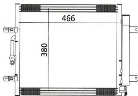
CAR MODEL: Fiat Palio 1.8 YEAR: 06-09 SIZE: 466x380x16
