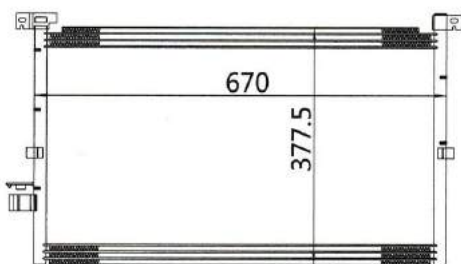
CAR MODEL: FORD MONDEO 2.0(03) YEAR: 03- SIZE: 670x377.5x16
