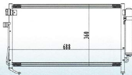
CAR MODEL: SUBARU FORESTER YEAR: 03-06 SIZE: 688×360×16
