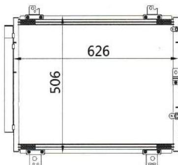
CAR MODEL: TOYOTA HIACE YEAR: 06- SIZE: 626x506x16
