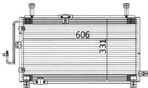
CAR MODEL: ISUZU D-MAX YEAR: 08~ SIZE: 606x331x16
