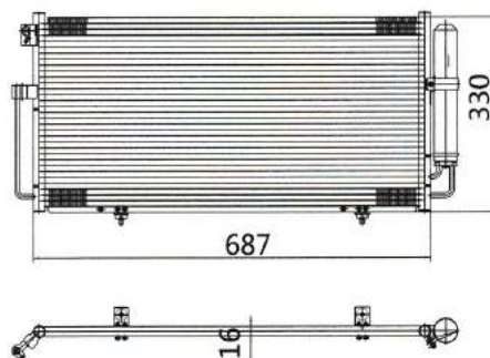
CAR MODEL: SUBARU Impreza GC# YEAR: 00-03 SIZE: 687×330×16
