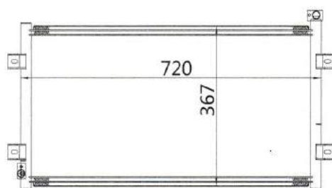
MODEL: 解放奥威 YEAR: SIZE: 720x367x20
