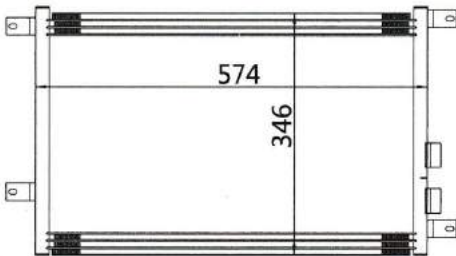
CAR MODEL: ALFA ROMEO 147 1.9 TD YEAR: 2001 SIZE: 574x346x16
