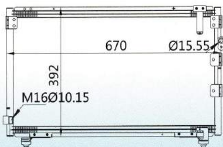
CAR MODEL: TOYOTA PICNIC/sport van YEAR: 96-01 SIZE: 670×392×16
