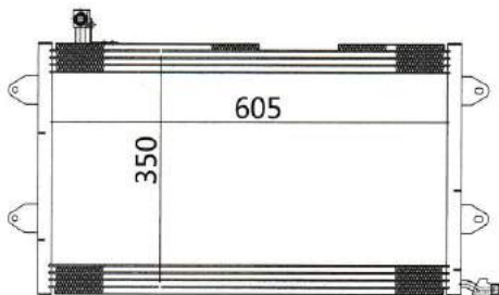
CAR MODEL: VW GOLF III YEAR: 93-96 SIZE: 605x350x16
