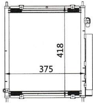
CAR MODEL: HONDA FIT 5D YEAR: 03- SIZE: 375×418×16
