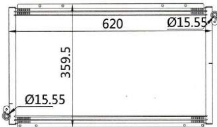
CAR MODEL: TOYOTA CELICA YEAR: 93-99 SIZE: 620×359×16
