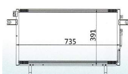
CAR MODEL: NISSAN PATHFINDER 3.3L YEAR: 98-00 SIZE: 391×735×16
