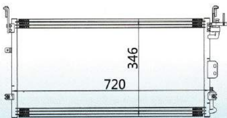
CAR MODEL: HYUNDAI SONATA YEAR: 02-04 SIZE: 720x346x16
