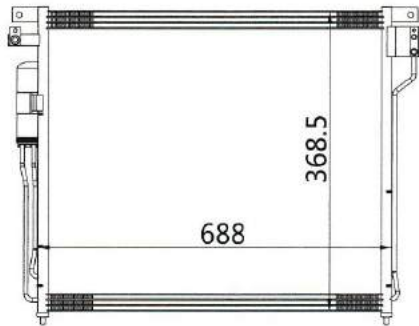
CAR MODEL: NISSAN XTERRA YEAR: 05-09 SIZE: 688×368.5×16
