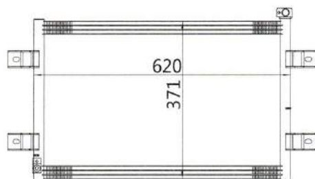
MODEL: 悍威 J5 重卡 YEAR: SIZE: 620x371x20
