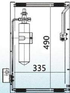
MODEL: 欧曼 YEAR: SIZE: 335x490x20
