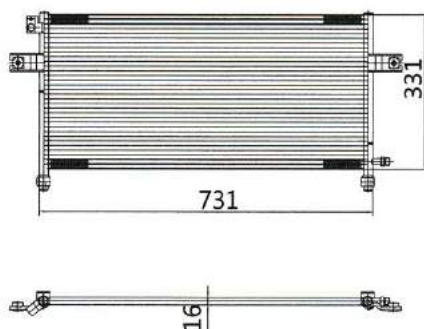
CAR MODEL: NISSAN FRONTIER YEAR: SIZE: 730×301×16
