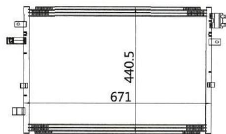
CAR MODEL: FORD MONDEO 2.5 / FORD MONDEO (00-) 2.0 YEAR: 2000 SIZE: 671x440.5x16
