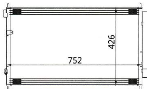
CAR MODEL: HONDA ODYSSEY YEAR: SIZE: 752×426×16
