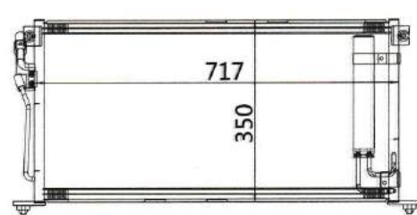
CAR MODEL: MITSUBISHI LANCER CH/2.0L YEAR: 04-07 SIZE: 717x350x16
