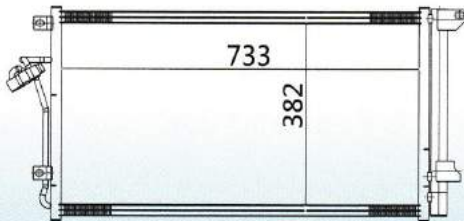
CAR MODEL: VOLKSWAGEN TOUAREG YEAR: 06- SIZE: 733x382x16
