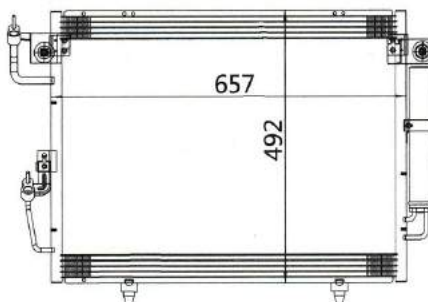
CAR MODEL: MITSUBISHI PAJERO YEAR: 98-09 SIZE: 657x492x16
