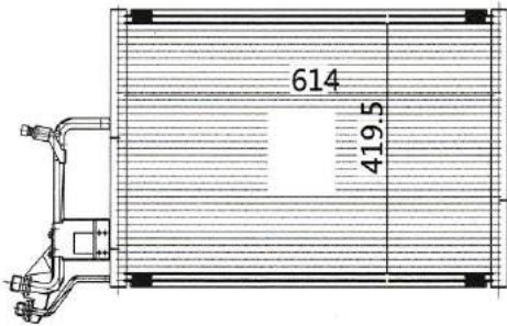
CAR MODEL: AUDI A4(20) YEAR: 94-97 SIZE: 614x419.5x20
