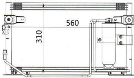
CAR MODEL: YEAR: SIZE: 560x310x20
