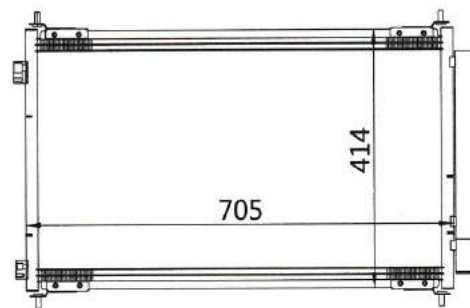
CAR MODEL: HONDA MDX-08 YEAR: SIZE: 705×414×16
