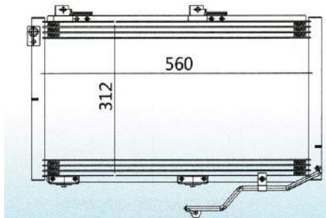
MODEL: 红旗三代 YEAR: SIZE: 560x312x20
