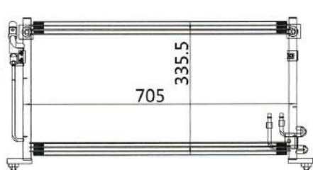
CAR MODEL: MITSUBISHI LANCER YEAR: 00-03 SIZE: 705x335.5x16
