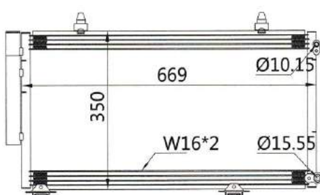
CAR MODEL: TOYOTA VIOS 04 YEAR: 04 SIZE: 669×350×16
