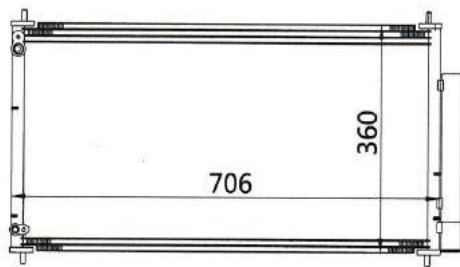
CAR MODEL: HONDA ACCORD YEAR: 2008 SIZE: 706×360×16
