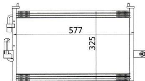
CAR MODEL: KIA MAXIMA/INFINITI YEAR: SIZE: 577x325x16
