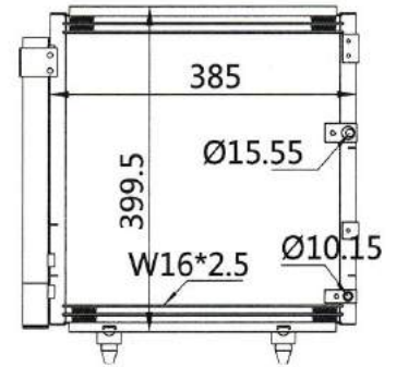
CAR MODEL: TOYOTA AVANZA(MT) YEAR: SIZE: 385×399×16
