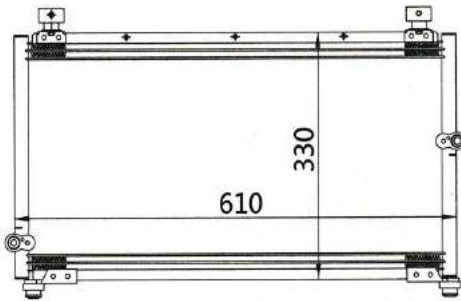
CAR MODEL: HONDA ACCORD YEAR: 93-97 SIZE: 610×330×16
