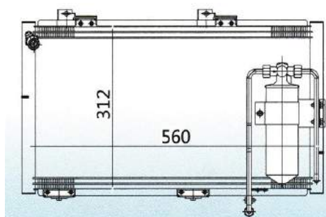
MODEL: 小红旗 YEAR: SIZE: 560x312x20
