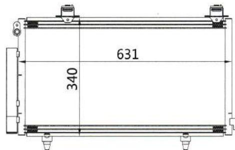
CAR MODEL: TOYOTA VIOS 03-05 YEAR: 03-05 SIZE: 631×335×16
