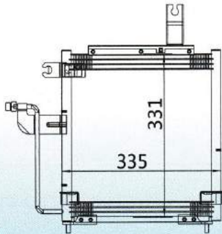
CAR MODEL: MAZDA DEMIO YEAR: 1996 SIZE: 335x331x16
