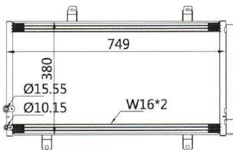
CAR MODEL : TOYOTA Camry ACV4# 06- YEAR: 05-10 SIZE: 749x380x16
