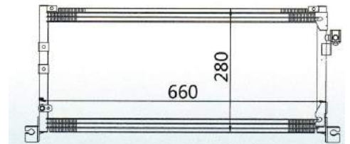
CAR MODEL: COROLLA YEAR: 99 SIZE: 660x280x16
