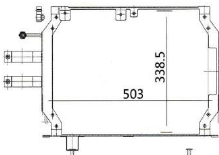
CAR MODEL: SUZUKI GAZELLE CS7100 YEAR: SIZE: 503x338.5x16
