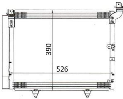
CAR MODEL: TOYOTA RUSH YEAR: SIZE: 526x390x16
