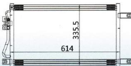
CAR MODEL: MITSUBISHI CHALLENGER K96W YEAR: 98-04 SIZE: 614x335.5x16
