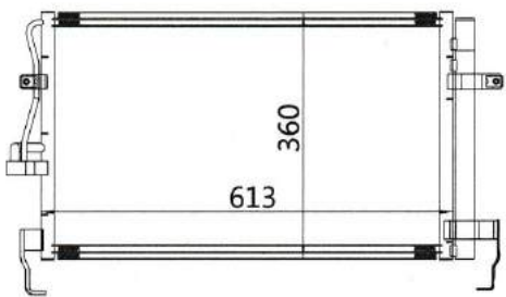
CAR MODEL: HYUNDAI ELANTRA /TIBURON YEAR: 01-07 SIZE: 613x360x16
