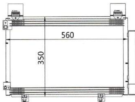
CAR MODEL: TOYOTA ECHO YEAR: SIZE: 560×350×16
