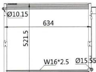
CAR MODEL: TOYOTA PRADO 4000 DOUBLE BLOCK/ TOYOTA GRJ120/Land Cruiser Prado GRJ120 02- YEAR: 03 SIZE: 634x521x16
