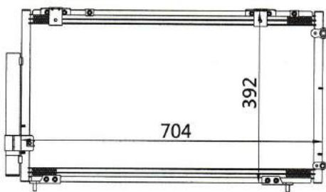
CAR MODEL: HONDA STREAM RN3 YEAR: 2000 SIZE: 704×392×16
