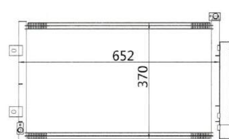
MODEL: 新悍威 (带瓶) YEAR: SIZE: 652x370x20
