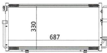
CAR MODEL: SUBARU IMPERZA YEAR: 04-07 SIZE: 687×330×16
