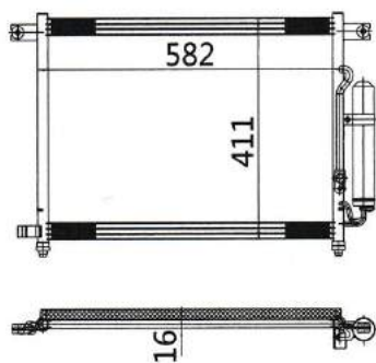
CAR MODEL: Daewoo Kalos YEAR: 07- SIZE: 582x411x16
