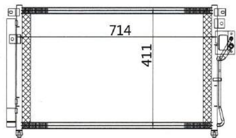
CAR MODEL : HN SANTA FE YEAR: 2007- SIZE: 714x411x16
