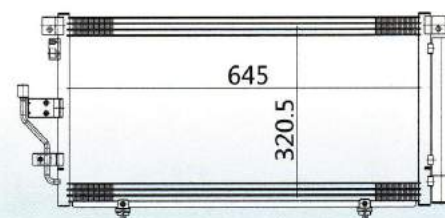
CAR MODEL: SUBARU Legacy B4 YEAR: SIZE: 645×320.5×16
