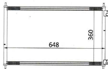
CAR MODEL: HONDA ACCORD YEAR: 02 SIZE: 648×360×16
