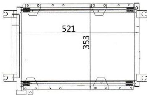
CAR MODEL: SUZUKI VITARA YEAR: SIZE: 521x353x16
