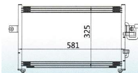
CAR MODEL: HYUNDAI ACCENT(X-3) YEAR: 94-99 SIZE: 581x325x16
