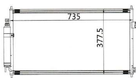
CAR MODEL: NISSAN X-Trail T30 YEAR: 00-03 SIZE: 735×377×16
