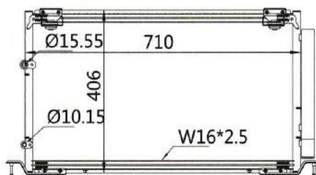
CAR MODEL: AVALON YEAR: 00-04 SIZE: 710×406×16
