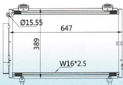
CAR MODEL: TOYOTA COROLLA/ALTIS (Middle East Version) /FIELDER/ RUNX/ALLEX/SPACIO/WILL VS 01- YEAR: 01 SIZE: 647x389x16
