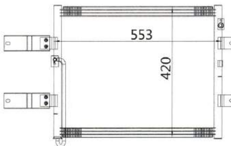
MODEL: YEAR: SIZE: 553x420x20
