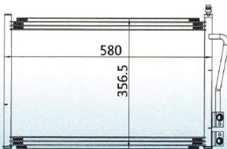
CAR MODEL: Ford Fiesta V YEAR: 01-04 SIZE: 580x356.5x16
