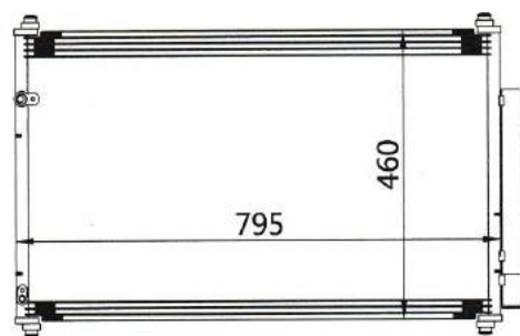
CAR MODEL: HONDA MDX-08 YEAR: 08- SIZE: 795×468×16
