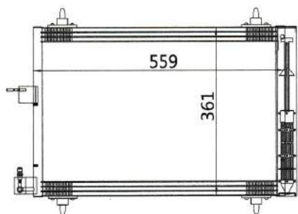
CAR MODEL: CITROEN C5 YEAR: 94-97 SIZE: 559x361x16
